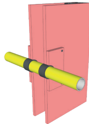
PEX-AL Pipe through 60 Min FRL Plasterboard Wall
