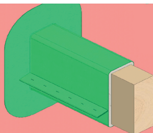
Wrap Green Collar Roll Around Plus 60 and Secure Using R31 Stapler and 12mm S/S Staples
